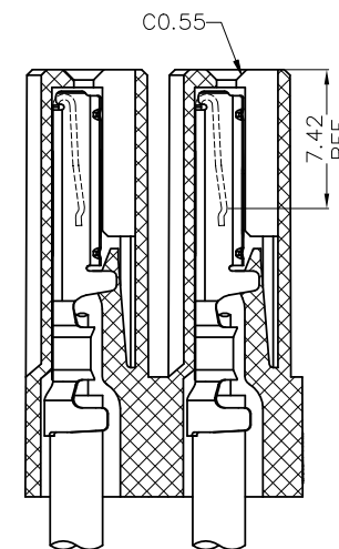
Terminal diagram
