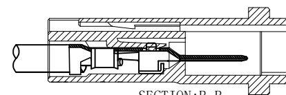
SECTION:B-B SCALE:1:1
