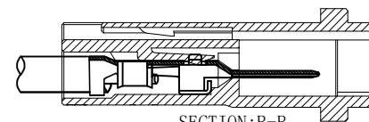
SECTION:B-B SCALE:1:1
