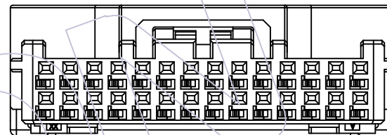
KEY-1 (28P)
