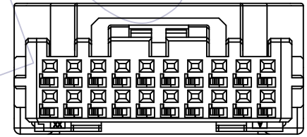
KEY-2 (20P)
