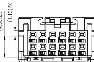
KEY-1 (12P)
