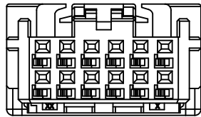
KEY-1 (12P)
