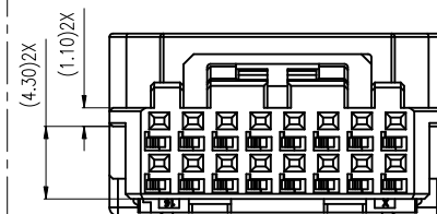
KEY-1 (16P)
