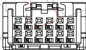
KEY-3 (12P)
