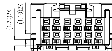
KEY-3 (12P)
