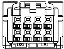
KEY-1 (8P)
