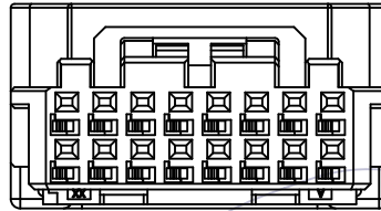
KEY-1 (16P)
