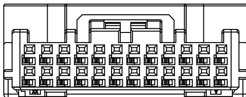
KEY-3 (24P)
