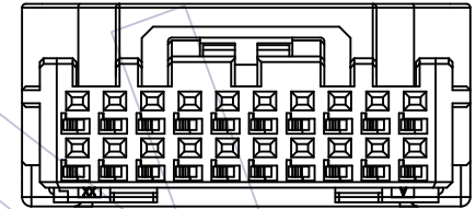
KEY-1 (20P)
