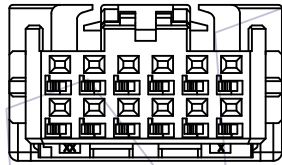
KEY-2 (12P)
