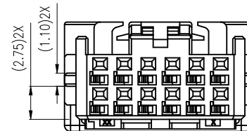
KEY-2 (12P)
