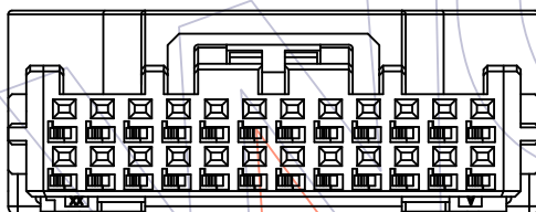
KEY-2 (24P)
