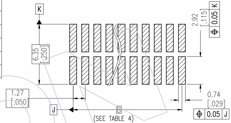
Recommended P.C.B Layout(Top Side) (PCB BOARD TOLERANCE±0.05)
