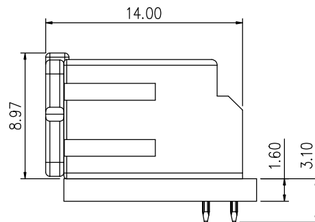
Side entry type (+WF2013-2WRHXXTT1)
