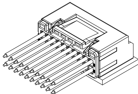
Side entry type (+WF2013-2WRHXXTT1)
