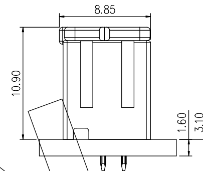
Top entry type (+WF2013-2WSHXXTT1)
