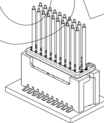
SMT type (+WF2013-2WMXXER1)
