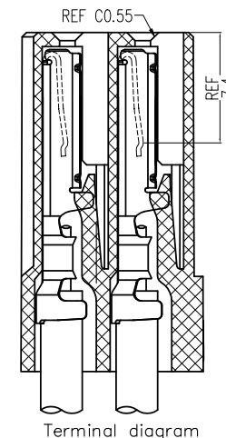
Terminal diagram
