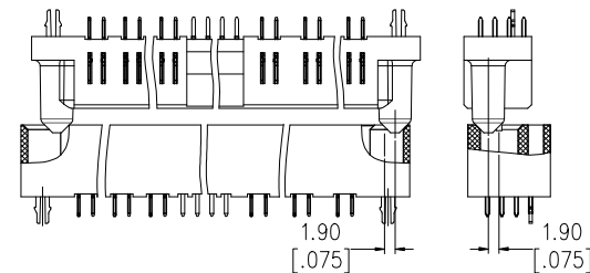
△3 Blind Mate Guide Ends SCALE: 1:2
