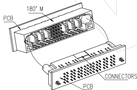
△3 Attempt to Match with 180° M
