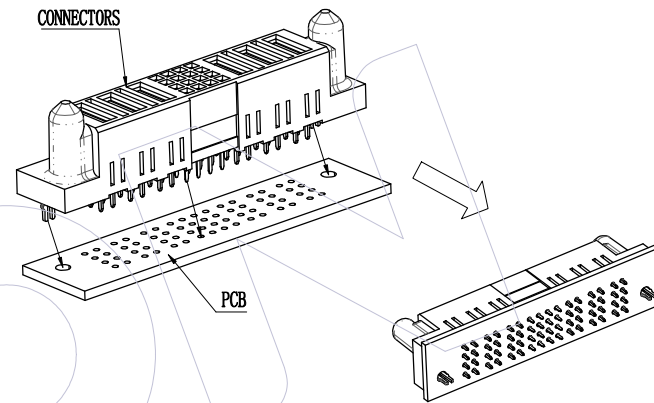
△3 PSP 180° DIP INSTALL CONNECTORS PCB
